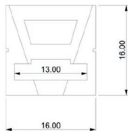
Flex LED in silicone 16×16 mm IP65.
